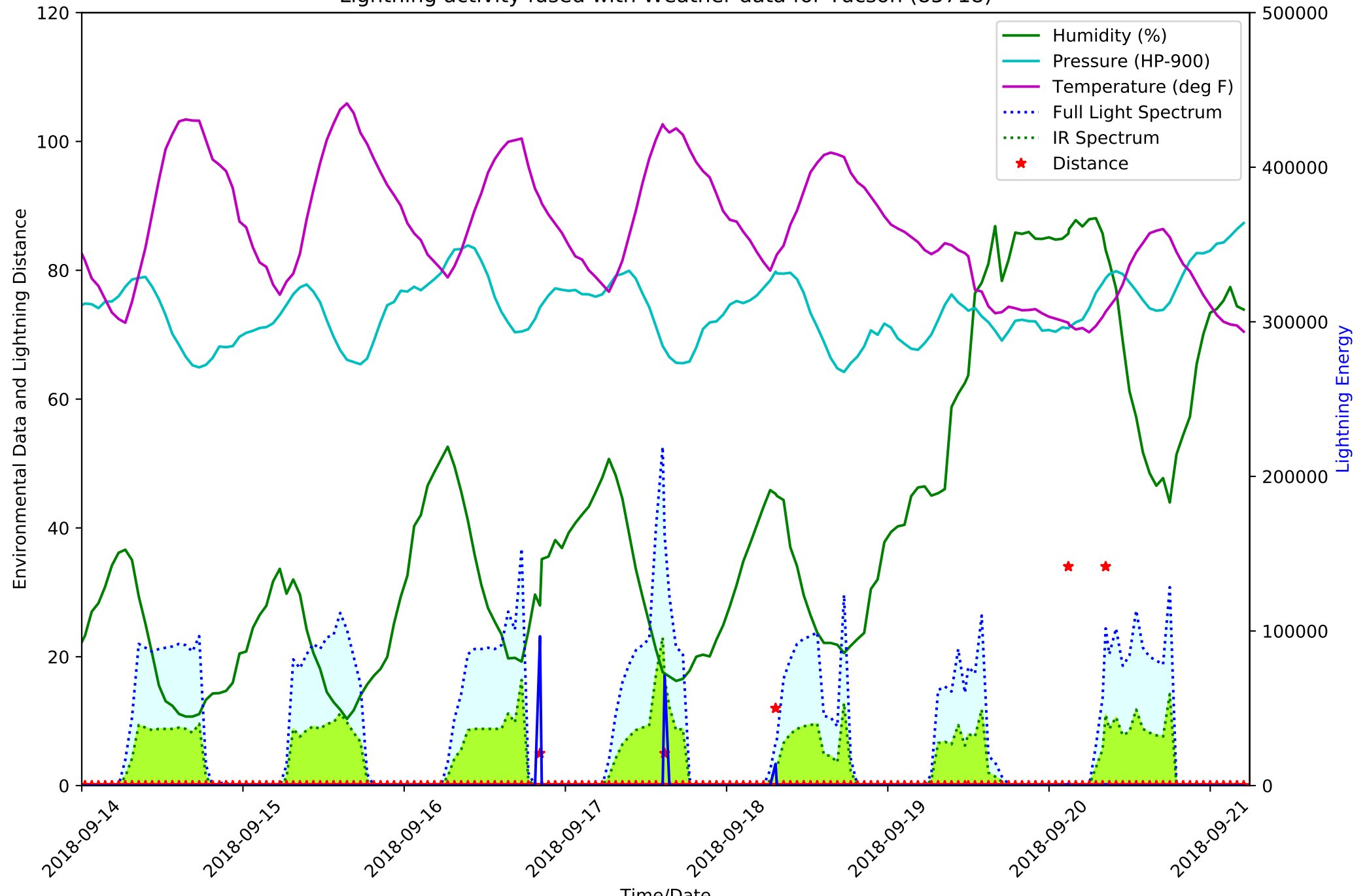
Lightning activity fused with Weather data for Tucson (85718)
