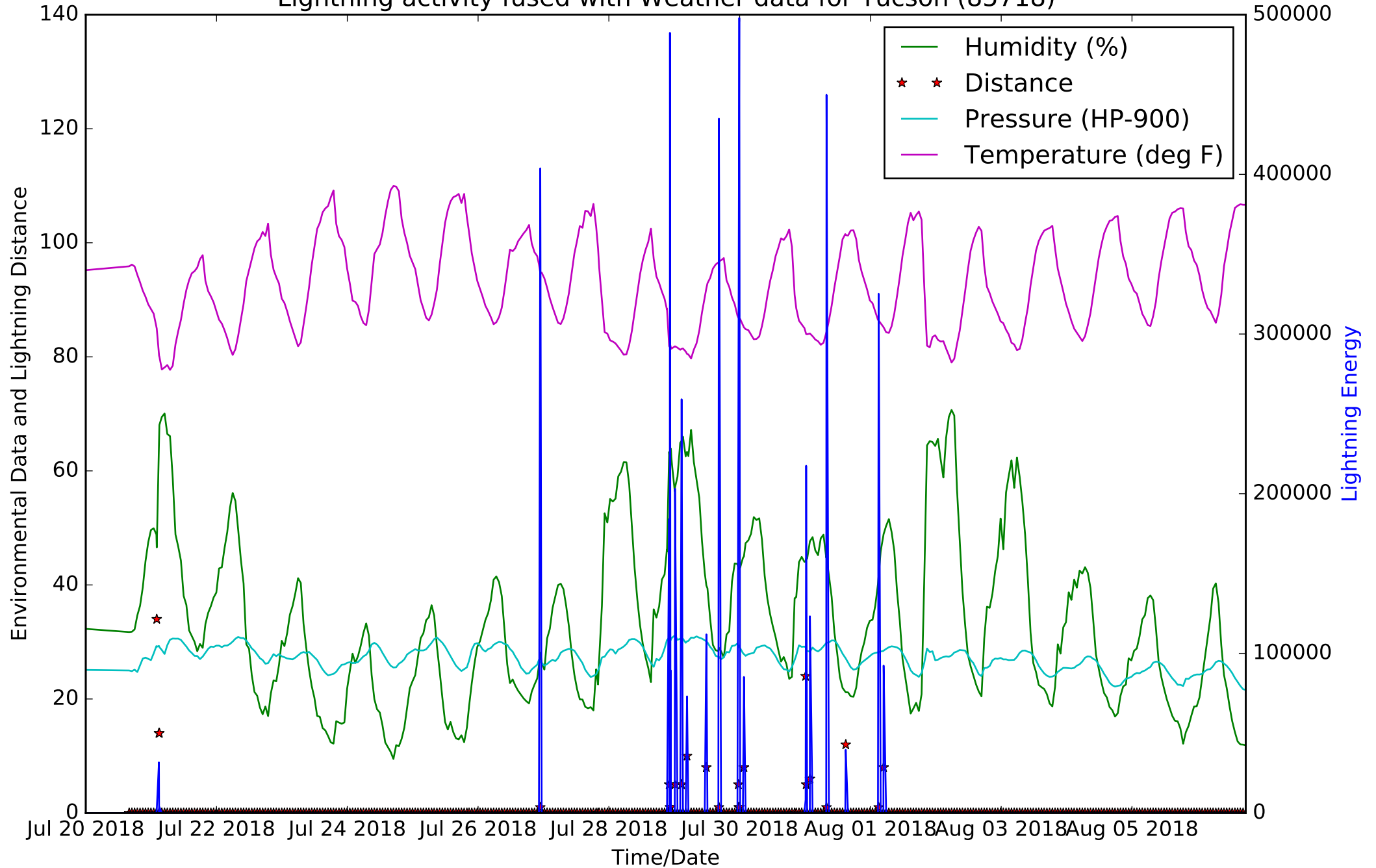
Lightning activity fused with Weather data for Tucson (85718)
