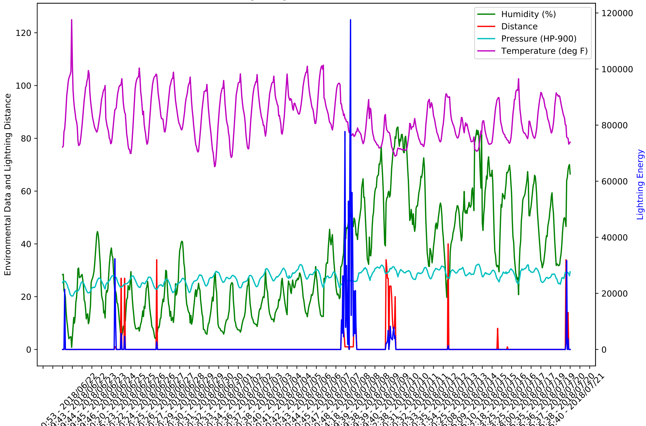
Tucson Lightning Sensor Data for 07/21/2018
