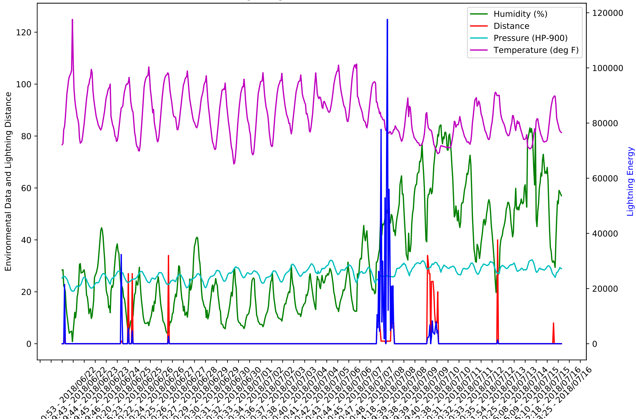
Tucson Lightning Sensor Data for 07/17/2018
